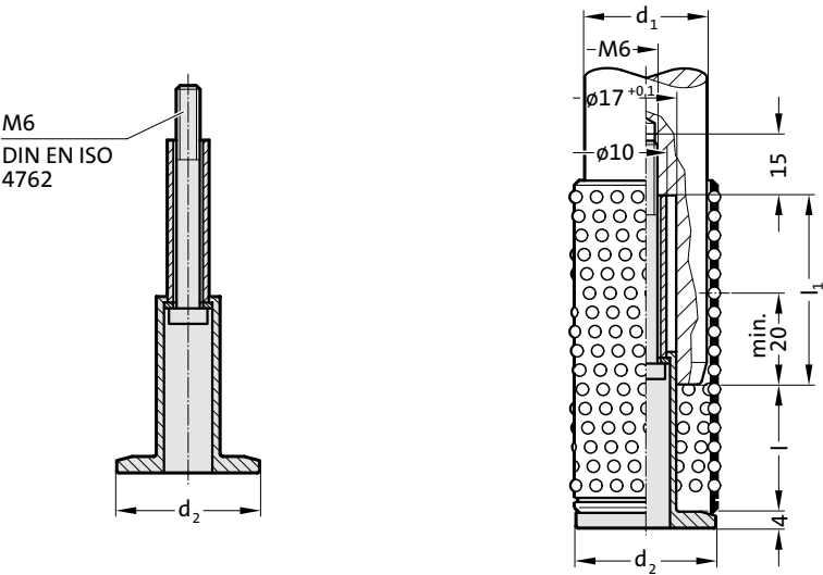
Mounting example
