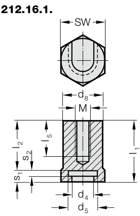
212.16.1 Spigot holder
