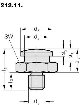
212.11. Coupling spigot with thread
