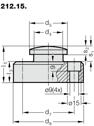
212.15. Coupling spigot with flange
