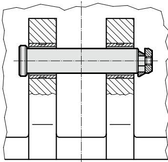
Mounting example
