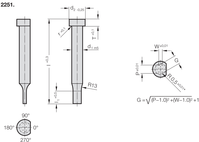
2251. Punch, stepped, rectangle with radiused corners, ISO 8020
