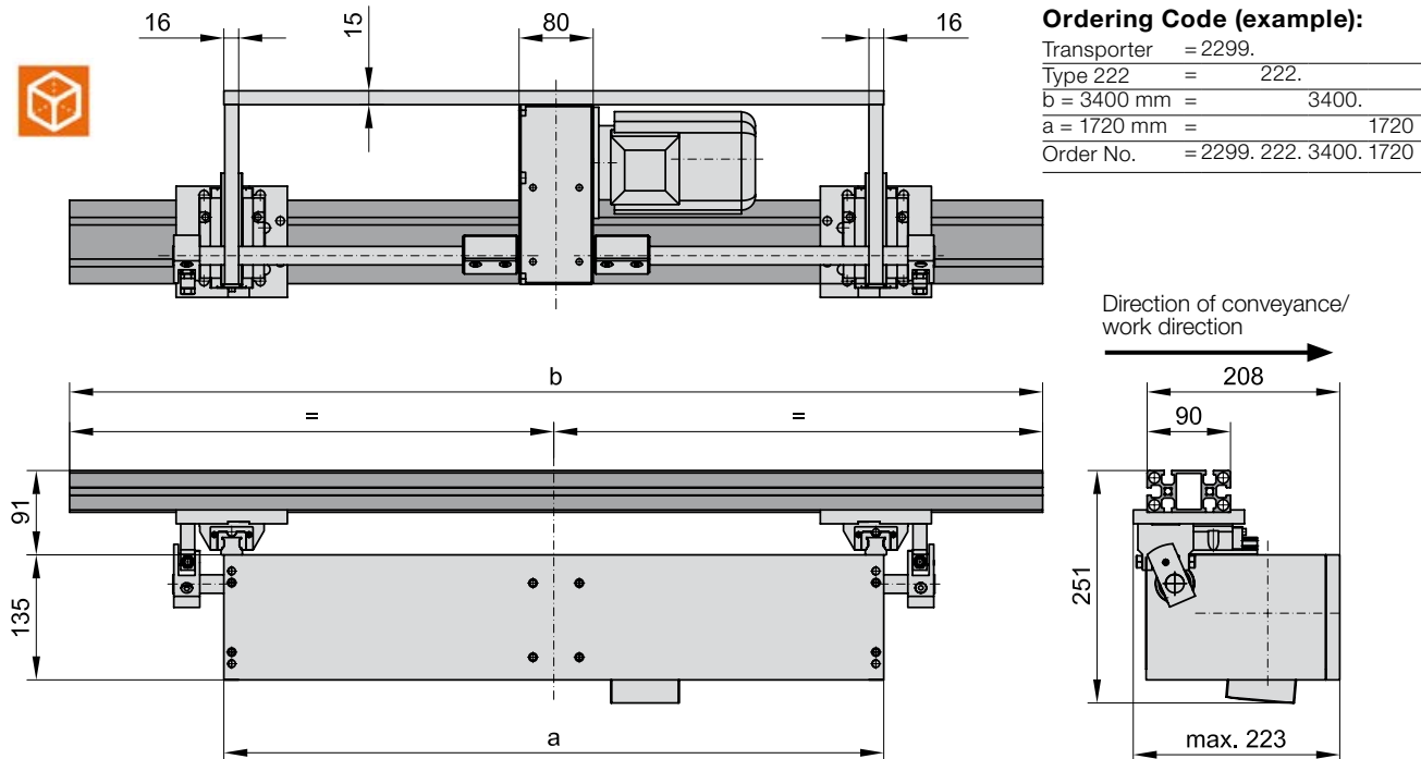
2299.222. horizontal centre gear position, two slides, with profile and support
