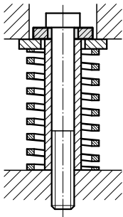
Mounting example
