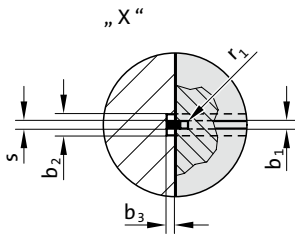
Mounting example
