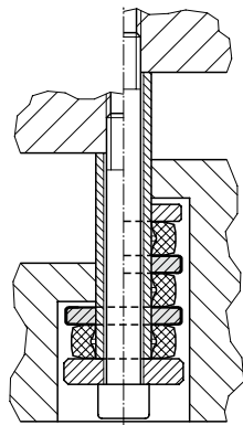
Mounting example
