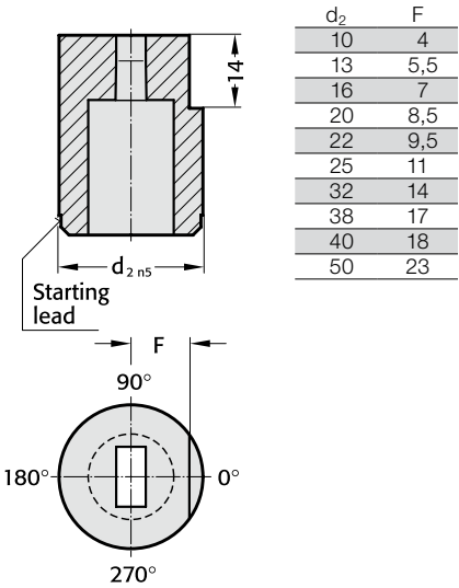
Anti-rotation element 5 (5)
