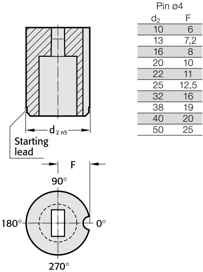
Anti-rotation element 2 (2)
