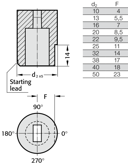
Anti-rotation element 6 (6)
