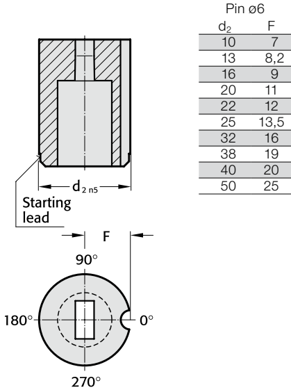
Anti-rotation element 3 (3)
