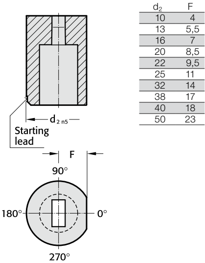
Anti-rotation element 4 (4)
