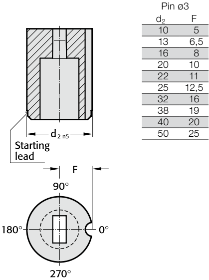
Anti-rotation element 1 (1)
