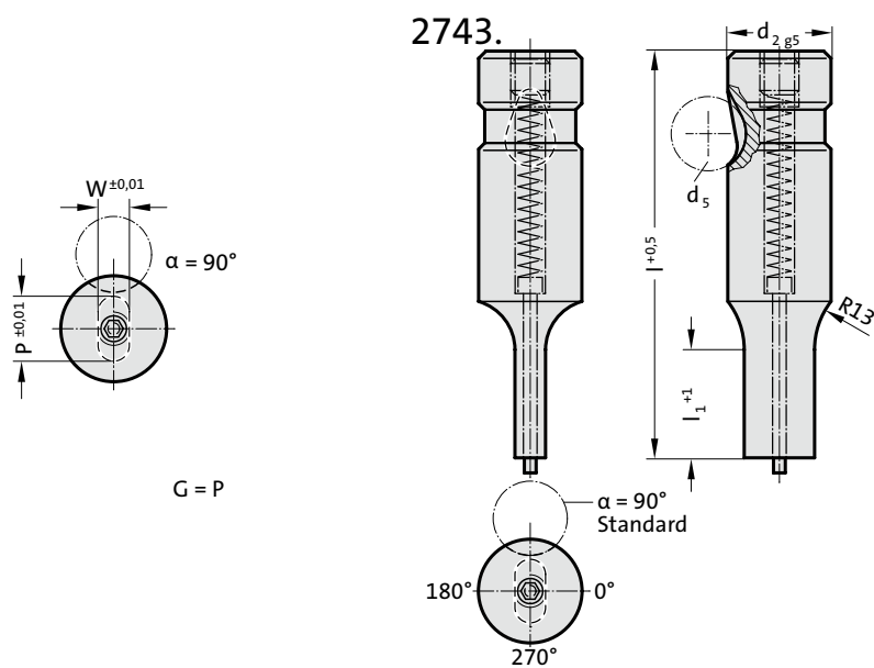
2743. Ball-Lock punch, stepped, slot, with ejector pin, heavy duty
