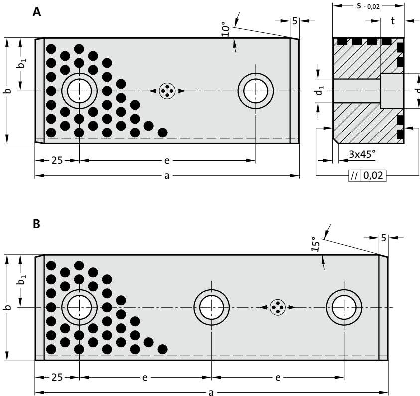
2962.75. Guide bar with two sliding surfaces, Bronze with solid lubricant, VDI 3357
