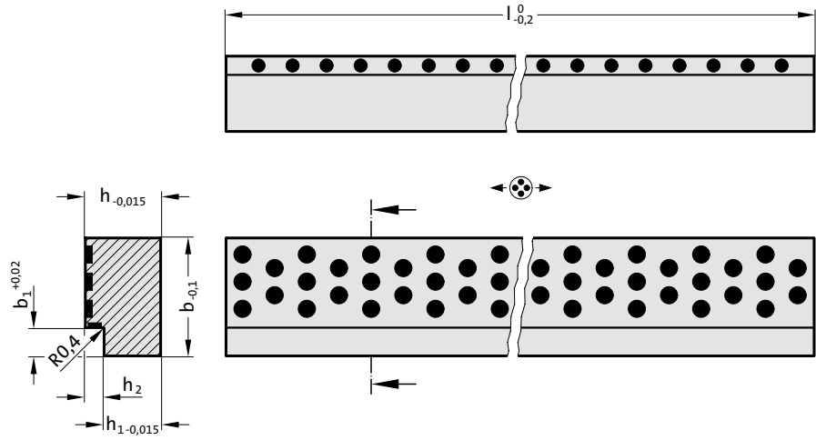
Material: Bronze with solid lubricant, oilless lubricating
