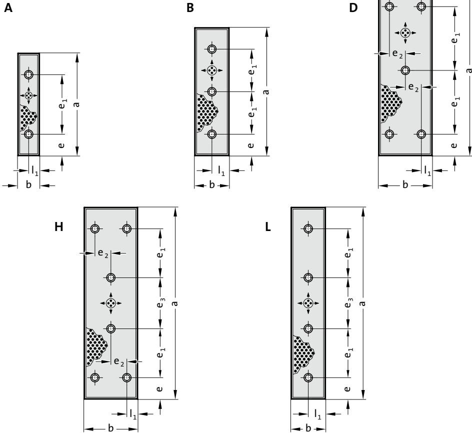
2962.85. Sliding pad, Steel with solid lubricant
