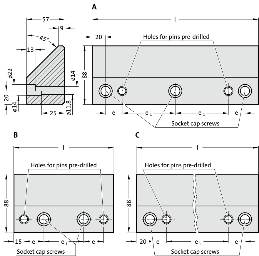
2965.82. Single-sided prismatic sliding block, Steel
