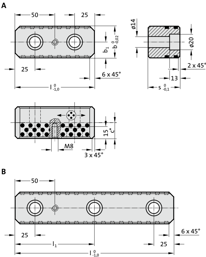
2966.72. Slide centre guide, Bronze with solid lubricant
