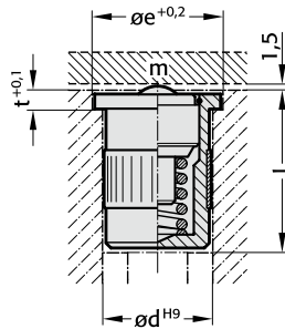
2198.33.Ball bearing insert with collar
