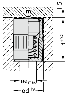
2198.32.Ball bearing insert without collar
