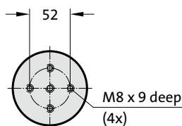
View X
