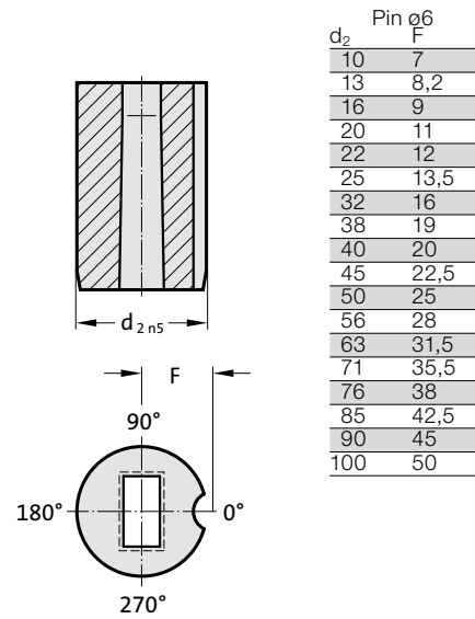
Anti-rotation element 3 (3)
