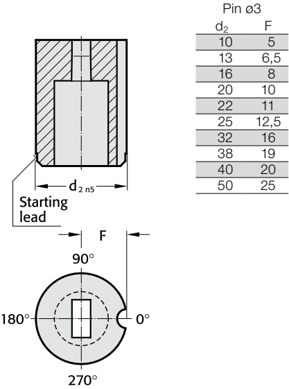
Anti-rotation element 1 (1)
