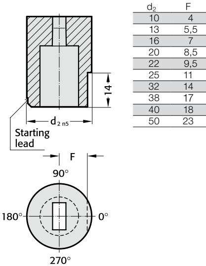
Anti-rotation element 6 (6)
