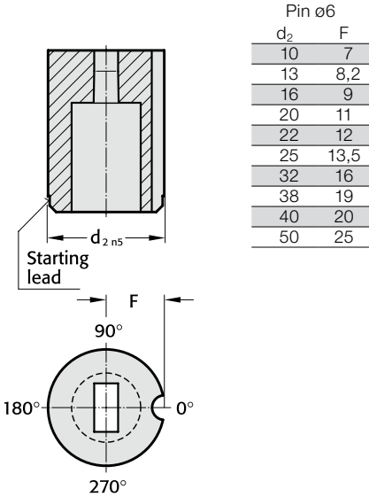
Anti-rotation element 3 (3)
