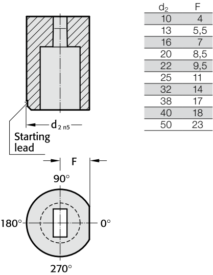
Anti-rotation element 4 (4)
