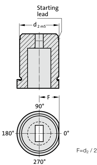
Anti-rotation element 4 (4)
