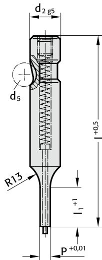
2712. Ball-Lock punch, stepped, round, with ejector pin, light duty
