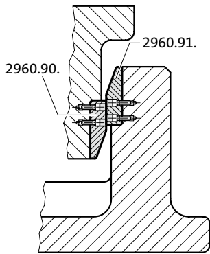
Mounting example
