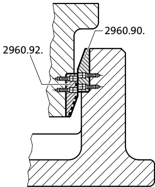
Mounting example
