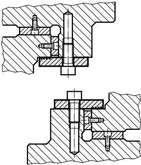
Mounting example
