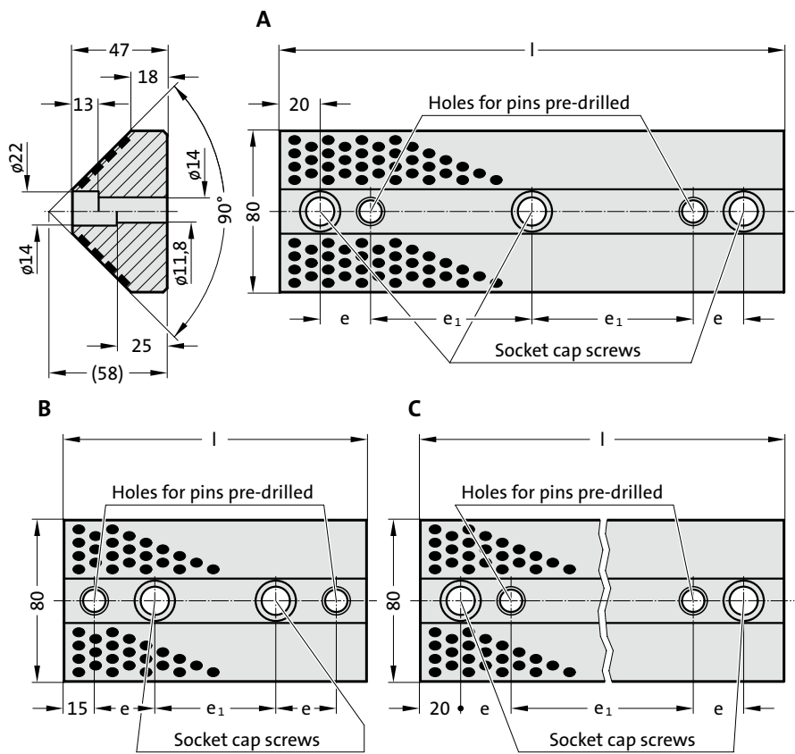
2963.80. Sliding block, Bronze with solid lubricant
